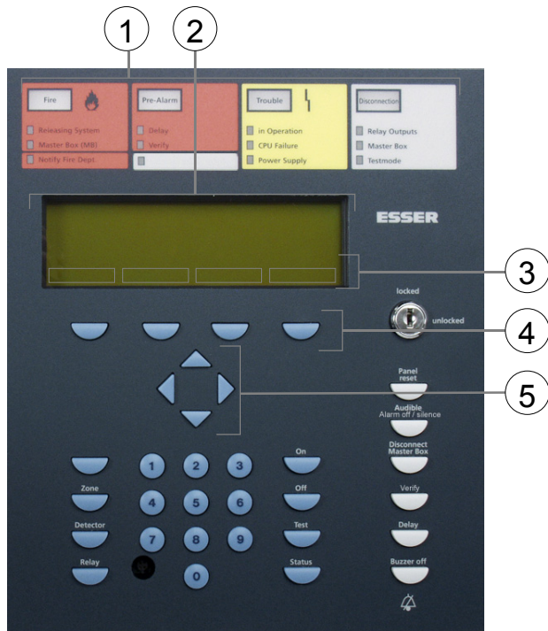
Fig. 4: Operating elements - keypad - display
