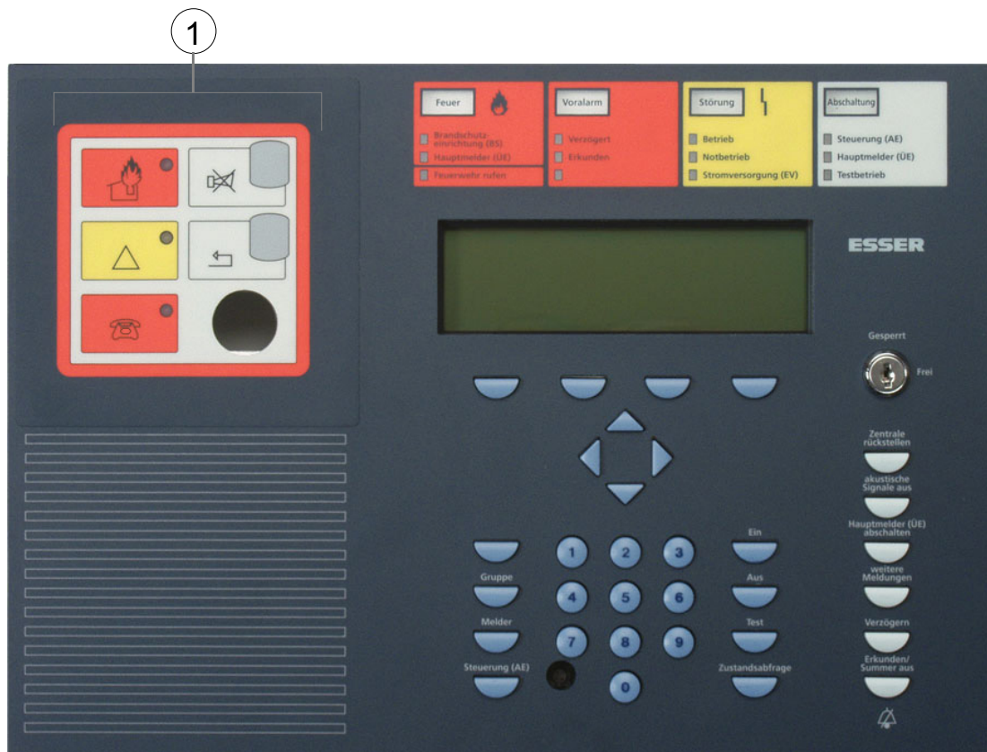
Fig. 10: panel front with integrated Fire department operating and indicating panel (FBA)
