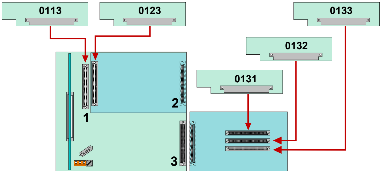
Fig. 48: Example: FACP IQ8Control
