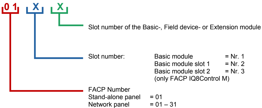
Fig. 48: Example: FACP IQ8Control
