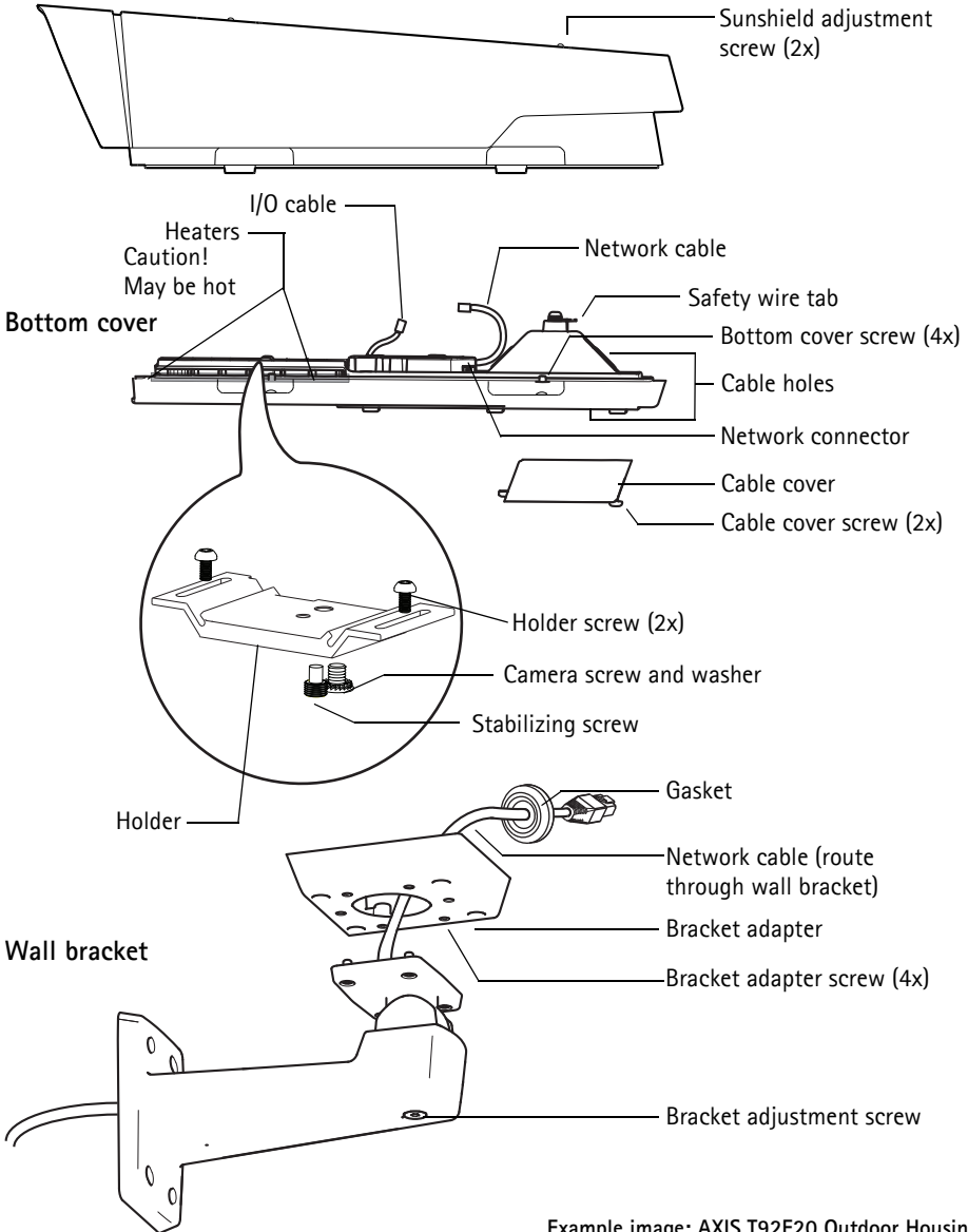
Example image: AXIS T92E20 Outdoor Housing
